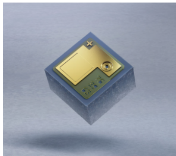
Chip die - 2 mW 850 nm VCSEL for high-volume applications and highly integrated sensors
